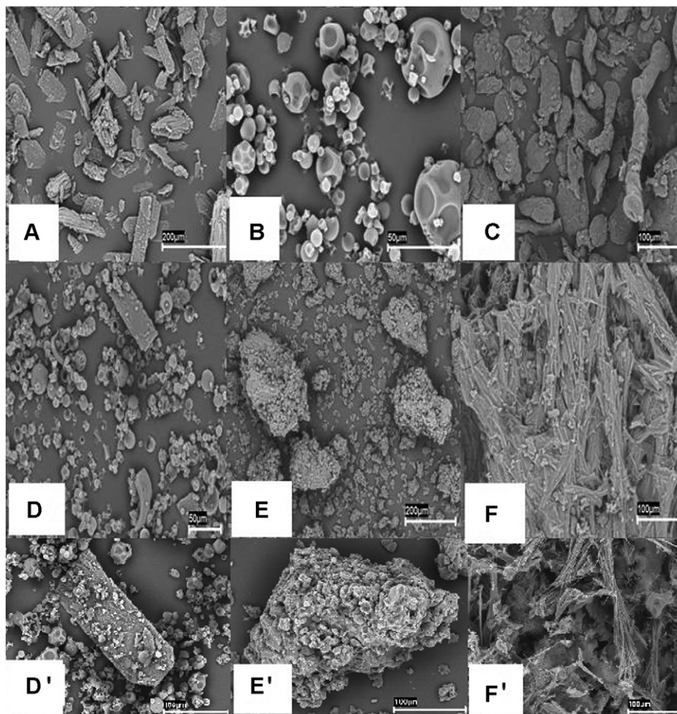
Fig. 3. Micrographs of the: A-BNZ; B-RMβCD; C-HPMC; ternary systems proportion 1:1 (D-PM; E-KN; F-EV); and the binary systems proportion 1:1 (D'-PM; E'-KN; F'-EV).
