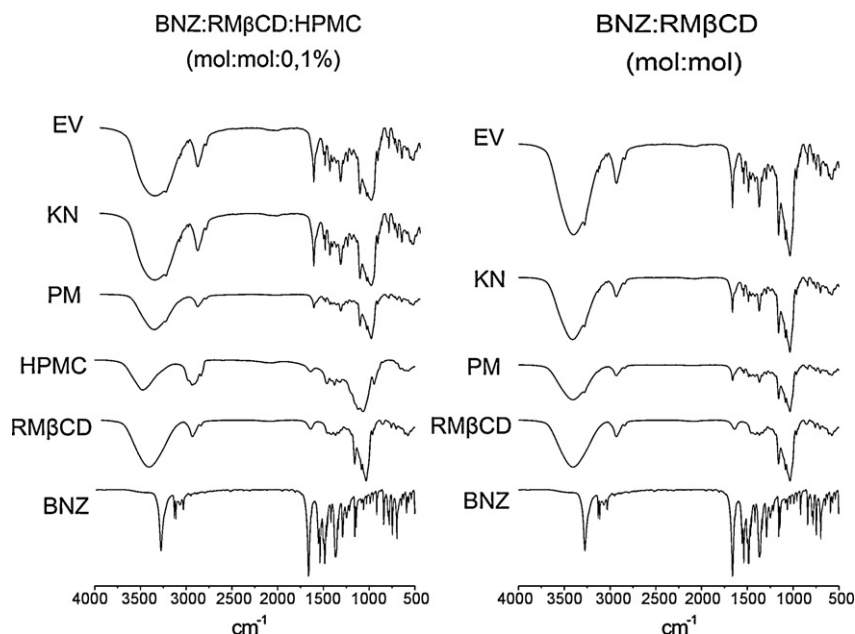
Fig. 4. FT-IR spectra of the binary and ternary systems: BNZ–RMβCD–HPMC sequence: BNZ, RMβCD, HPMC, PM, KN and EV; BNZ sequence: RMβCD, BNZ, RMβCD, PM, KN and EV.
