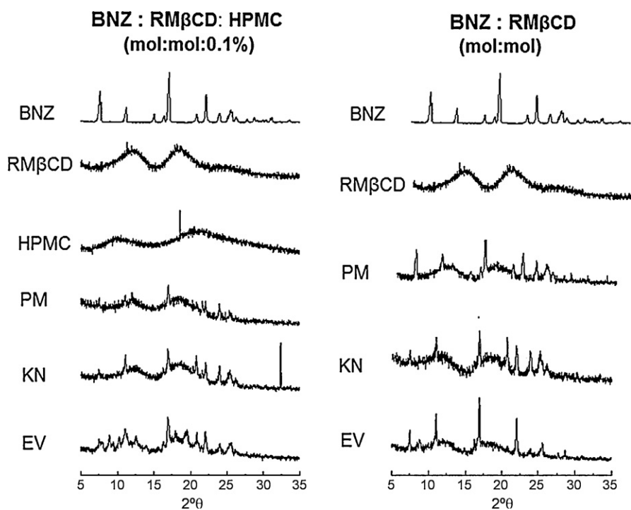
Fig. 2. Diffractograms of BNZ, HPMC, RMβCD, binary and ternary systems.
